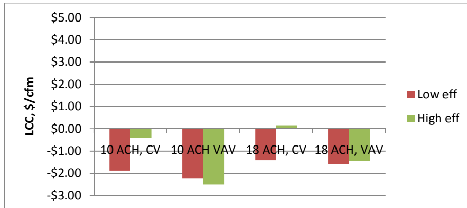
Figure 16. 15-year life-cycle cost, CTZ 12
