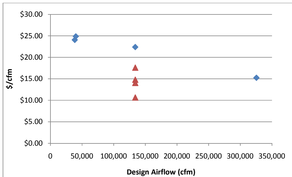
Figure 3. Cost data from four major lab retrofits
