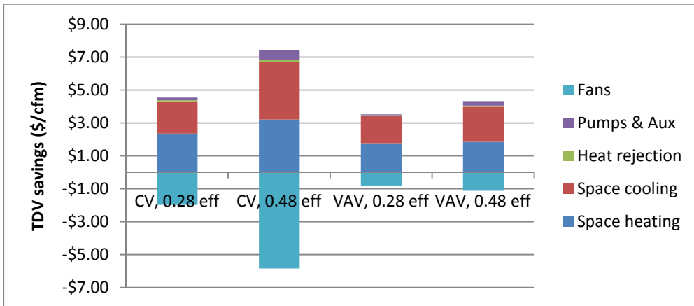
Figure 11. 15-year energy savings by end-use, CTZ 12, 18 ACH
