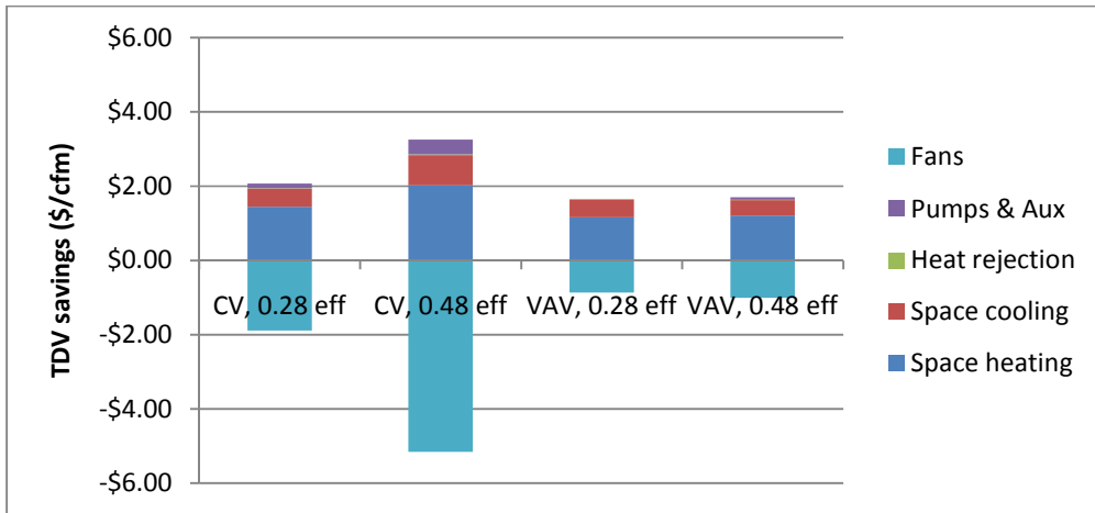
Figure 7. 15-year energy savings by end-use, CTZ 3, 18 ACH
