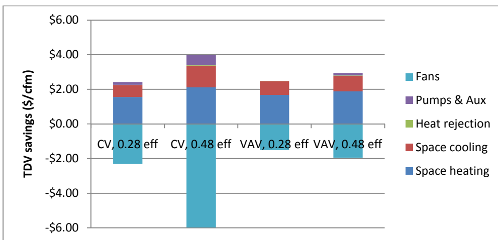
Figure 5. 15-year energy savings by end-use, CTZ 3, 10 ACH
